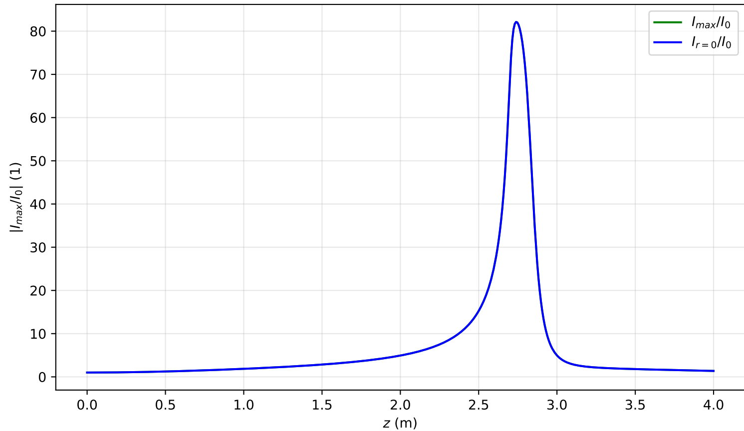
I_{max}(x = 0, y = 0, z)/I_0 , P_{in}=1.2P_{cr} , artificial time
